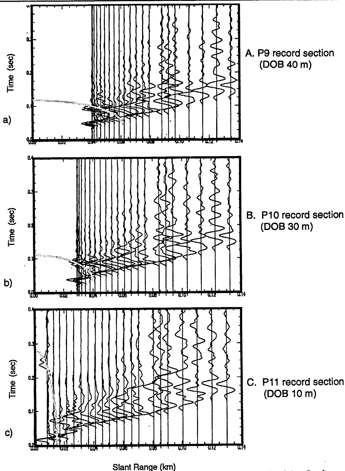
Figure 7. Record section plots of surface acceleration along the length of the Grefco Dicapperl test best (see the long linear array in Figure 1). The data are presented as a function of slant range to facilitate determination of seismic velocities. The observed extent of surface spall is denoted by the hatched line.
