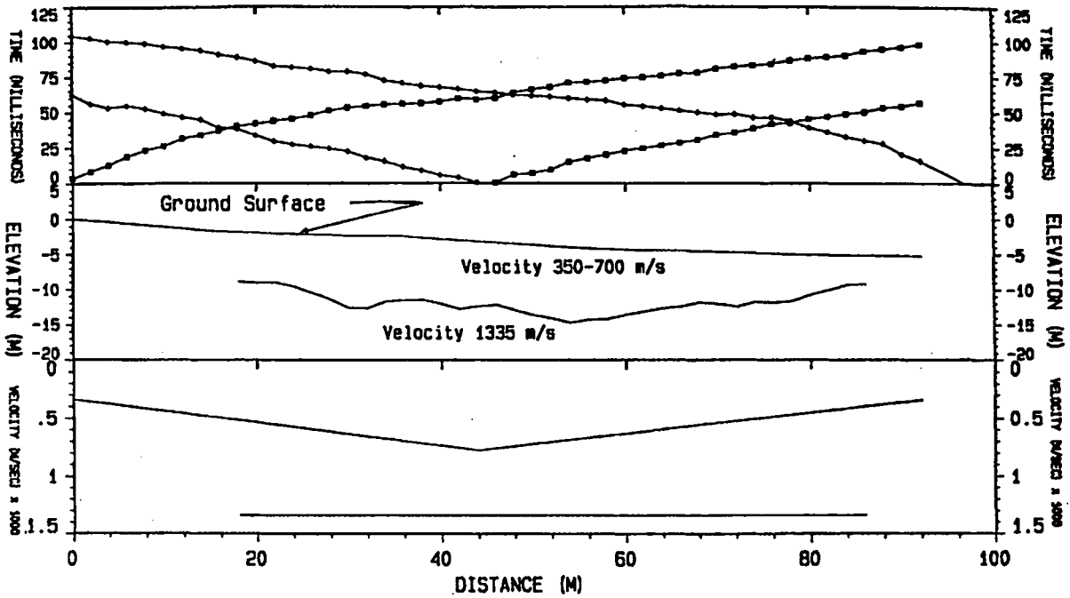
Figure B-3. Velocity model.
