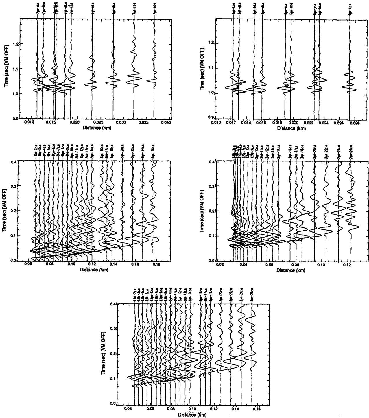
Figure 4. Section plot of perlite #5, 6, 7 data.
