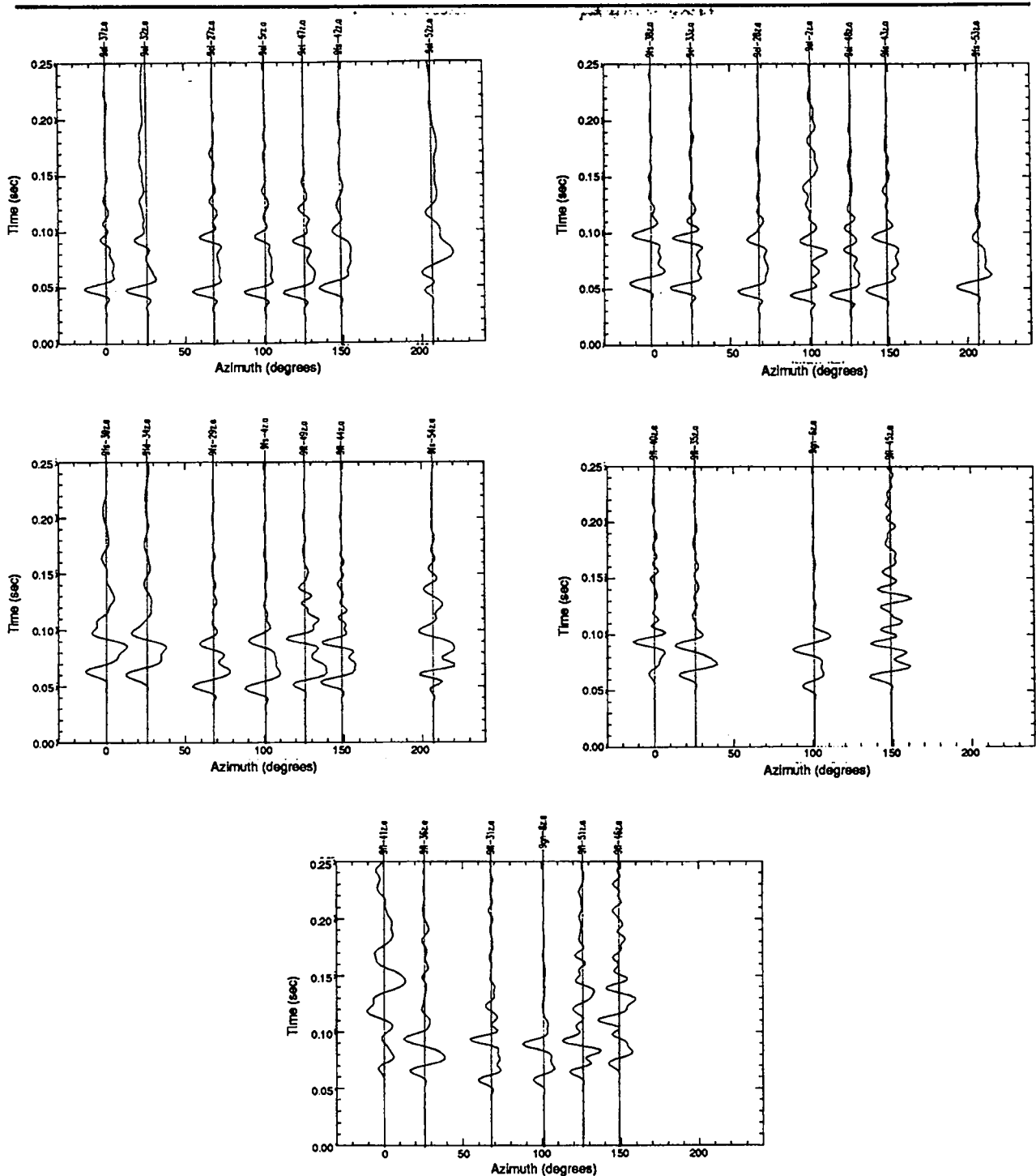
Figure 8. The azimuthal variation of the waveforms is shown for a) 5-m range, b) 10-m range, c) 20-m range, d) 30-m range, and e) 40-m range. At 5 m, the spall initiation time is nearly identical at all azimuths. At increasing ranges, the first motion is delayed in time at increasing and decreasing angles away from the major joint orientation near 0 deg. (see Figure 1). Spall dwell time decreases both with increasing range and increasing azimuth away from the major joint orientation.
