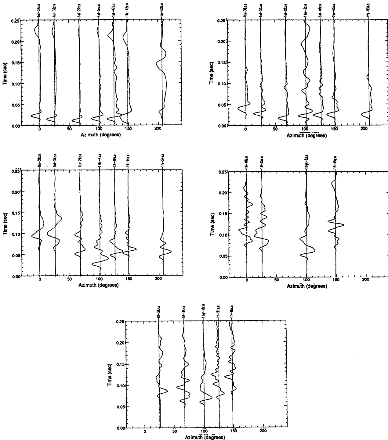
Figure 10. The azimuthal variation of the waveforms is shown for a) 5-m range, b) 10-m range, c) 20-m range, d) 30-m range, and E) 40-m range. At 5 m, the spall initiation time is nearly identical at all azimuths. At increasing ranges, the first motion is delayed in time at increasing and decreasing angles away from the major joint orientation near 0 deg. (see Figure 1). Spall dwell time decreases both increasing range and increasing azimuth away from the major joint orientation.
