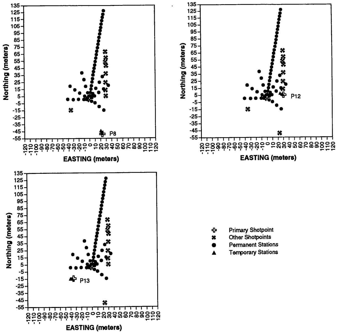
Figure 11. Experiment Layout Perlite #8, 12, 13.
