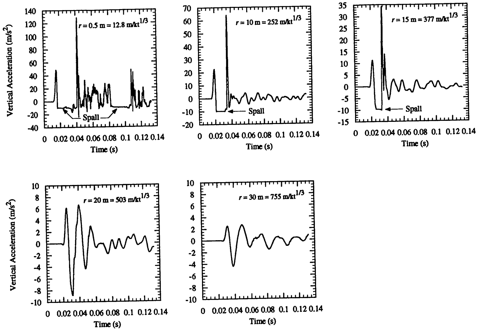
Figure C-5. Computed vertical acceleration ( m/s^2 ) at 5-cm depth as a function of time at 0.5, 10, 15, 20, and 30 m from SGZ in the two-dimensional calculation of 143 lb Unigel™ at 12 m DOB. The clear -1 g spall signal is apparent in the stations out to ~20 m (~500 m/kt^{1/3} ) range.
