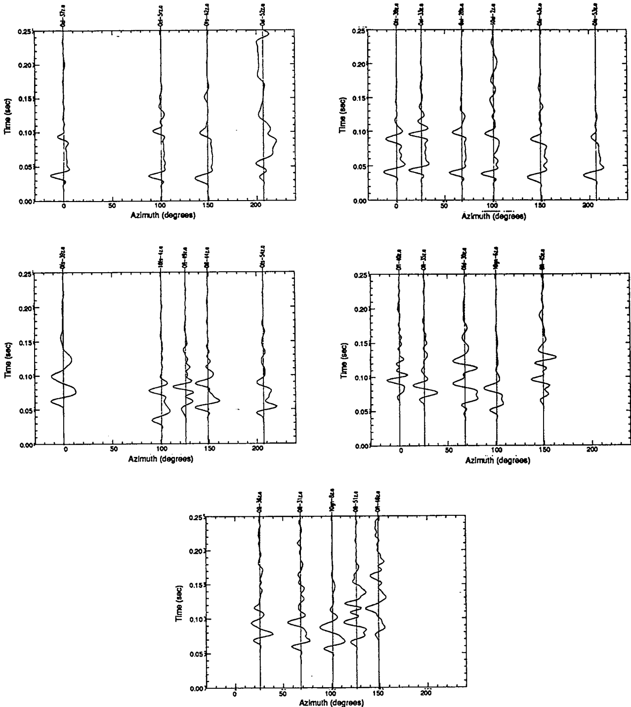
Figure 9. The azimuthal variation of the waveforms is shown for a) 5-m range, b) 10-m range, c) 20-m range, d) 30-m range, and E) 40-m range. At 5 m, the spall initiation time is nearly identical at all azimuths. At increasing ranges, the first motion is delayed in time at increasing and decreasing angles away from the major joint orientation near 0 deg. (see Figure 1). Spall dwell time decreases both increasing range and increasing azimuth away from the major joint orientation.
