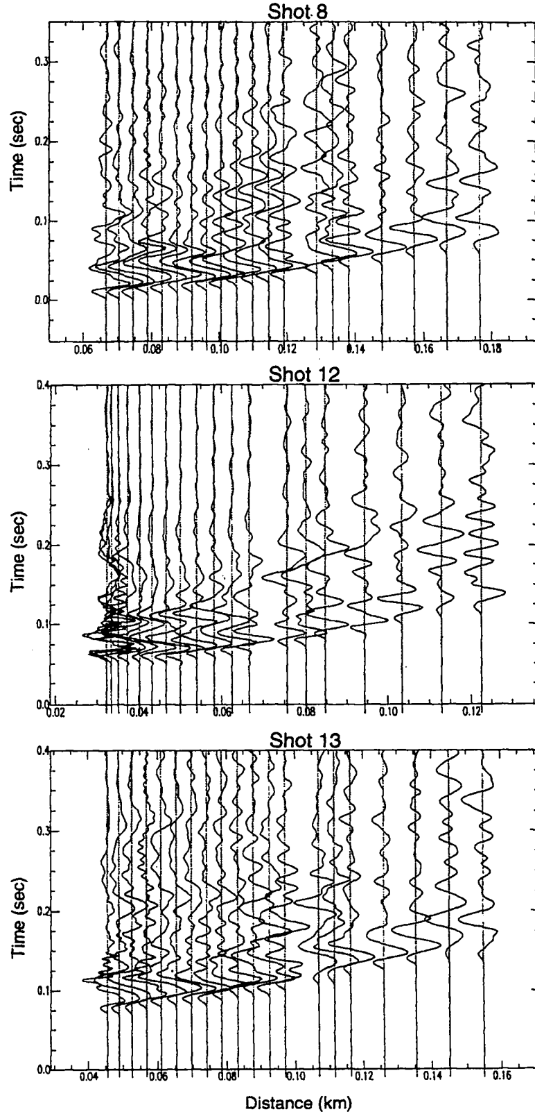
Figure 13. Record Section Plot of Perlite #8, 12, 13.
