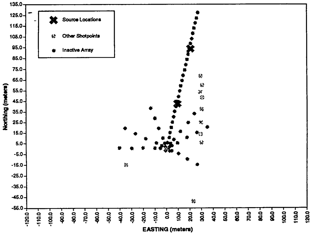
Figure B-1. Refraction survey layout
