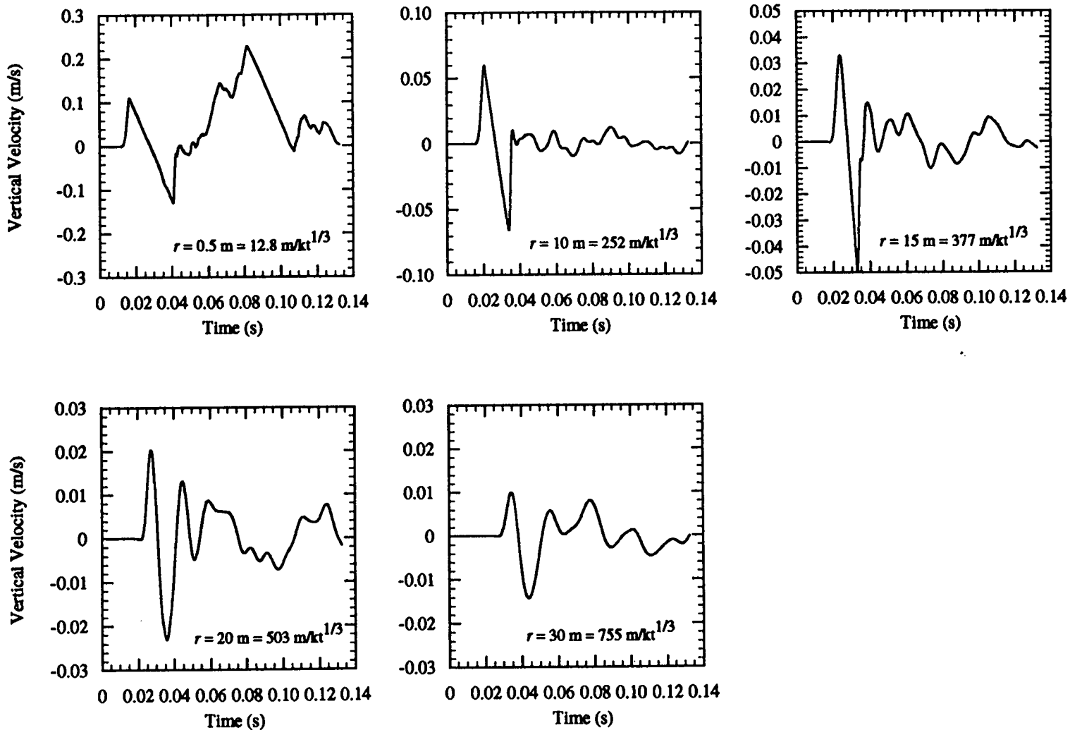
Figure C-6. Computed vertical velocity records at 5-cm depth at 0.5, 10, 15, 20, and 30 m from SGZ in the two-dimensional calculation of 143 lb Unigel™ explosive buried at 12 m in perlite. The regions of constant negative slope in the top three plots correspond to a ballistic free-fall phase associated with the surface spall.
