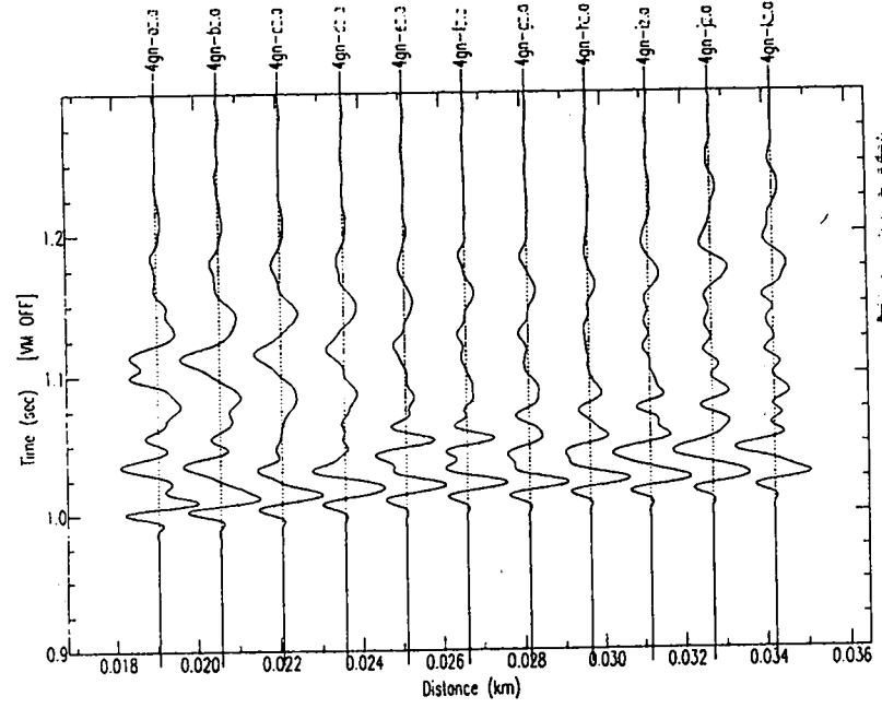
Figure 3. Section plot of Perlite #1, 2, 3, 4 data.
