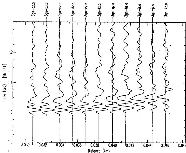
Figure 3. Section plot of Perlite #1, 2, 3, 4 data.
