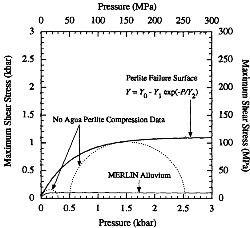
Figure C-2. Maximum shear stress (kbar) versus confining pressure (kbar) for the Grefco No Agua perlite data [2] and for MERLIN alluvium [5]. A failure surface of the form given in Equation 1 was "eyeballed" to fit the perlite data. The shear behavior of the No Agua perlite may differ from that of the Socorro perlite. According to this model, the maximum shear stress ( at a given confining pressure) is notably greater for perlite than for alluvium.
