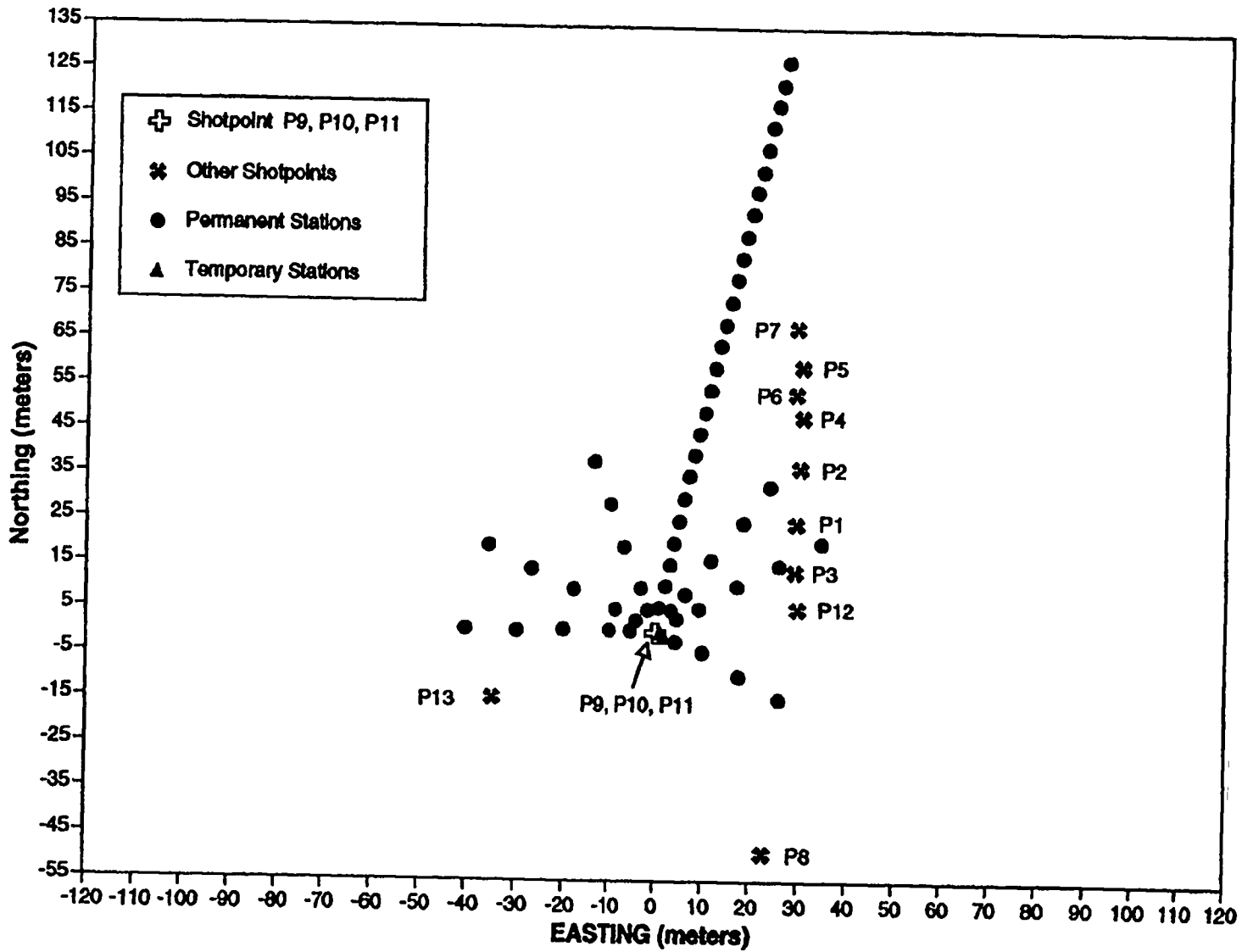
Figure 5. Experiment layout P9, P10, P11.
