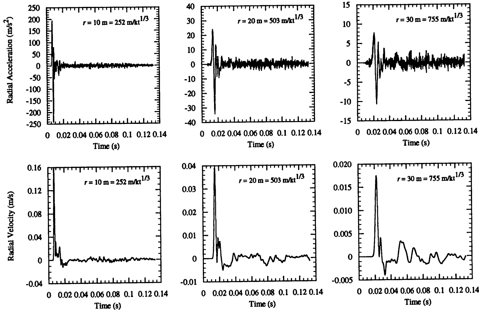
Figure C-8. Computed free-field radial acceleration (m/s 2 ) at shot level as a function of time at 10, 20, and 30 m from the shot point (top row), and free-field radial velocity (m/s) at shot level at the same ranges (bottom row) in the two dimensional calculation of 143 lb Unigel™ at 12-m DOB in perlite.
