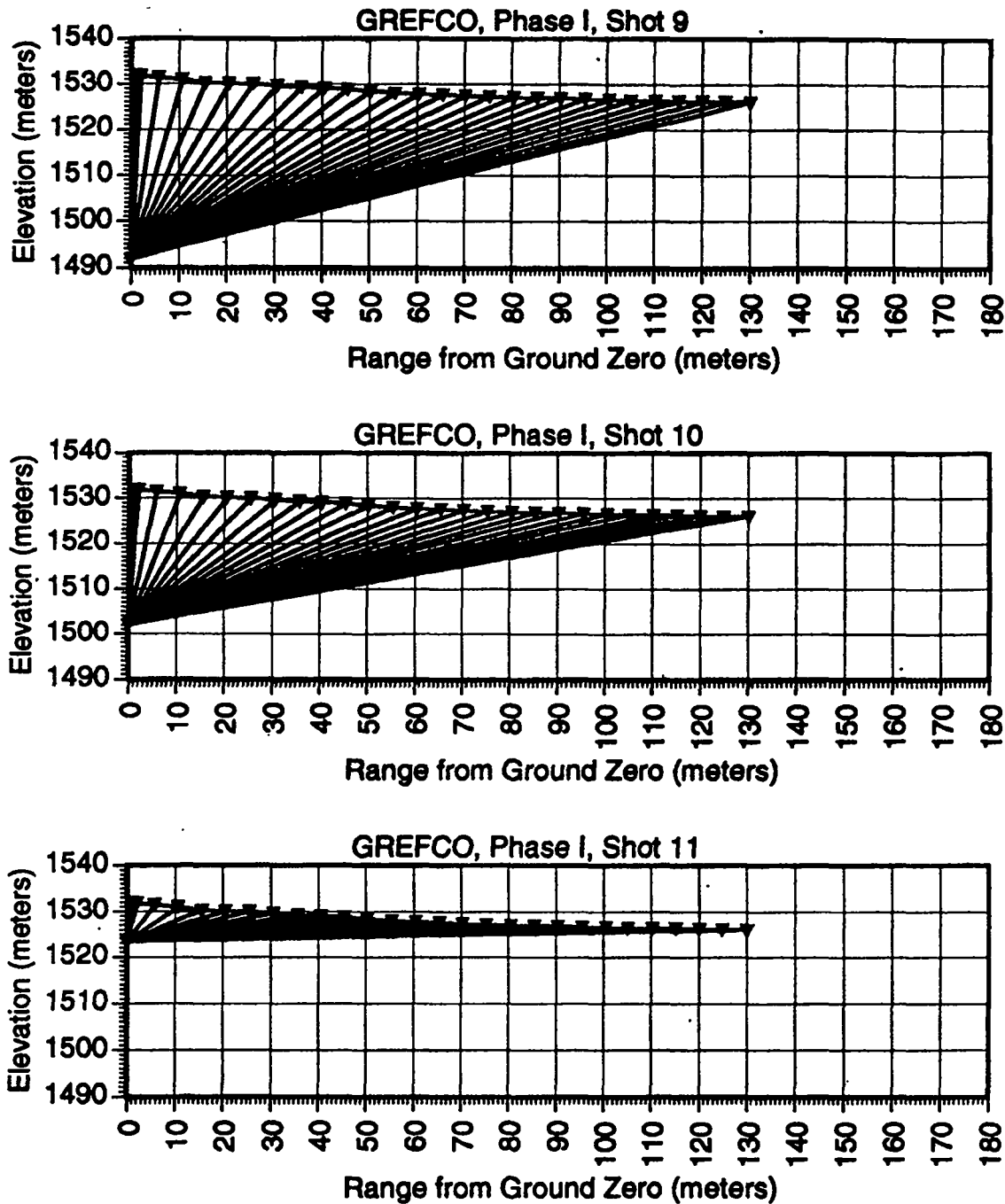
Figure 6. Ray path geometry for shots P9 (a), P-10 (b), and P11 (c). The shot depth of burial (DOB) strongly affects the incidence angle of the wave front at the stations composing the long linear array (see Figure 1).
